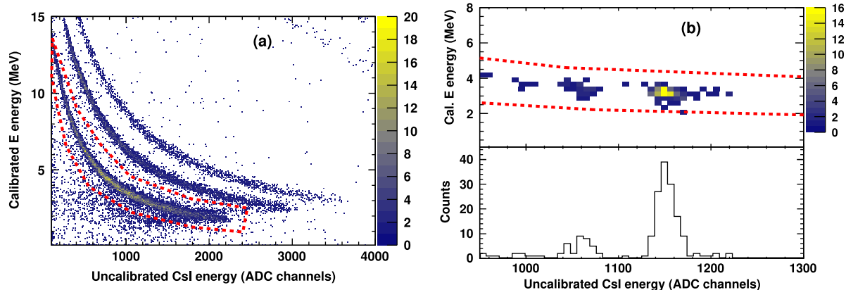
Fig. 11. (a) HiRA PID plot for reaction data using one CsI crystal and its corresponding E silicon detector. The y -axis is calibrated energy in the E detector, and the x -axis is uncalibrated CsI energy in units of ADC channels. Protons (within the red-dashed line) can clearly be identified, even though the CsI energy is uncalibrated. (b) The top panel is the HiRA PID for the same CsI crystal as in (a), this time showing the scattering data (zoomed in to the relevant region). The red-dashed line is the same proton gate as in (a). The bottom panel is a projection of the top panel onto the x -axis. Two peaks can clearly be seen: the higher energy peak corresponds to proton elastic scattering off carbon, and the lower energy peak is from inelastic scattering ( E^*(^{12}\text{C}) = 4.439 MeV).
