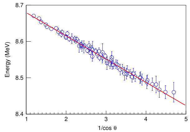
Fig. 8. Example energy distribution with statistical error bars for the 8.785 MeV peak across many pixels in a single telescope according to different values of 1/\cos\theta , as well as the corresponding fit.
