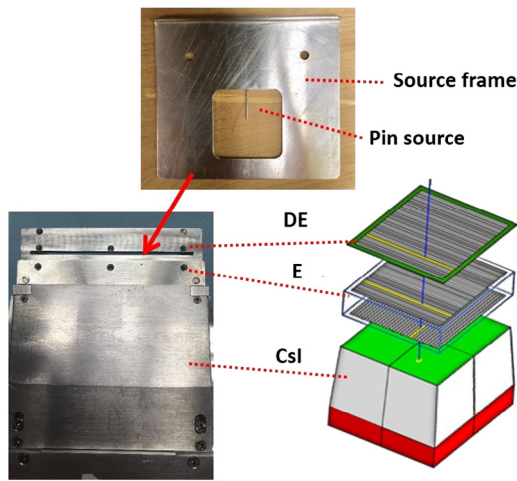
Fig. 1. HiRA telescope assembly. On the bottom left is a side-view photograph of a HiRA telescope. On the bottom right is a cartoon of the detectors contained within the telescope. Dotted red lines connect the detectors in the cartoon to their approximate positions in the telescope. On the top of the figure is the pin source frame with the pin source installed. The pin source slot is located between the DE and the E detector as indicated by the thick red arrow.
