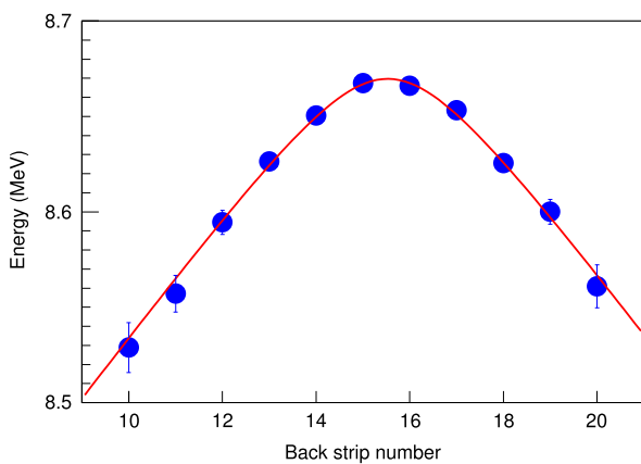
Fig. 7. Example energy distribution with statistical error bars of the 8.785 MeV peak for different pixels across the central front strip. The corresponding fit (using Eq. (2)) is shown in red. (For interpretation of the references to colour in this figure legend, the reader is referred to the web version of this article.)
