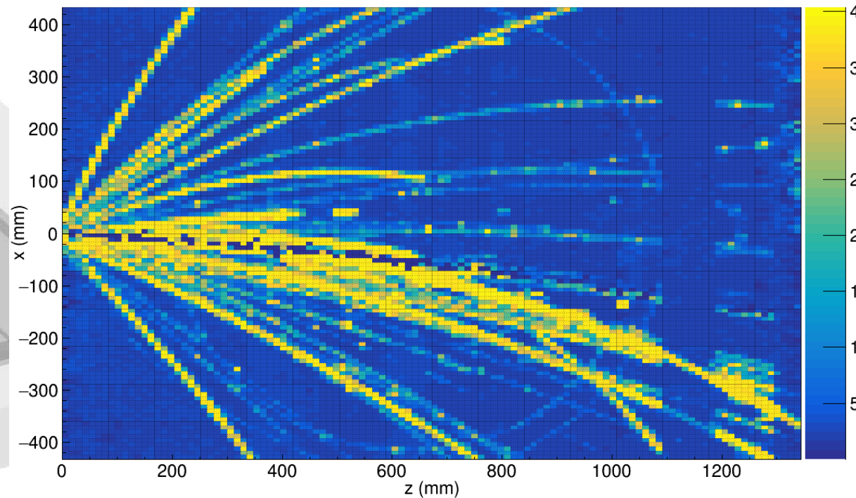
Run#2376 - Event ID: 148 (Gain not calibrated) - Top view
