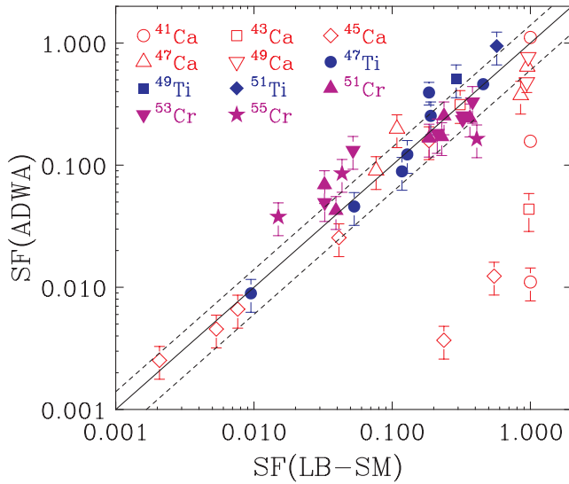
FIG. 2 (color online). Comparison of experimental spectroscopic factors, SF(ADWA) , to predictions from large-basis shell-model for the Ca, Ti, and Cr isotopes, SF(LB-SM) . Complete basis with the interaction GXPF1A is used in the theoretical calculations. The solid line indicates perfect agreement between data and predictions. Dashed lines represent \pm 40\% deviations from the solid line.
