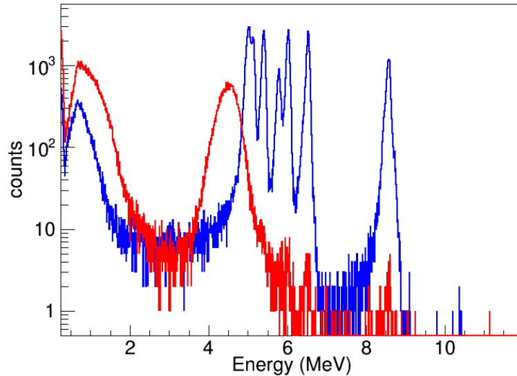
Figure 2: Calibrated alpha-particle spectrum obtained by combining data of HiRA strips of an entire telescope (32 strips). The blue spectrum is obtained without the use of the Sn/Pb absorber, while the red one is obtained when the Sn/Pb absorber is placed at the entrance window of the telescope. The latter is affected by straggling effects, broadening the observed peaks.
