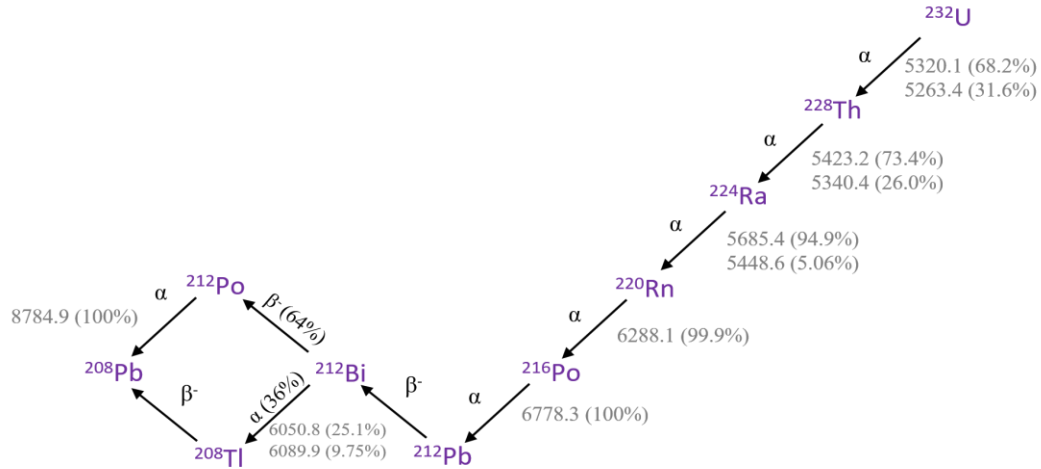
Figure 1: The decay scheme of ^{232}\text{U} . Alpha and beta decays are indicated. In the case of the alpha-decay, kinetic energies (MeV) of the emitted alphas and the corresponding emission probabilities are shown. The decay chain ends with ^{208}\text{Pb} .
