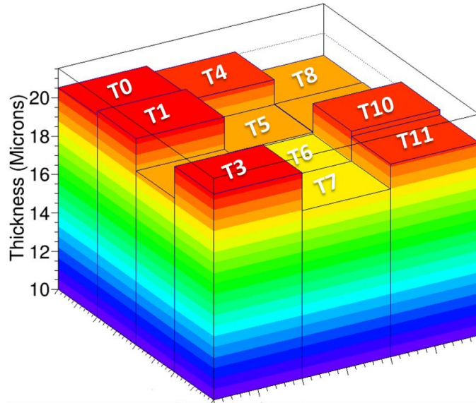
Figure 6: Thickness mapping of the Sn/Pb foils (for each telescope) obtained by means of the described analysis. Telescopes are numbered from 0 to 11 as shown by the labels.
