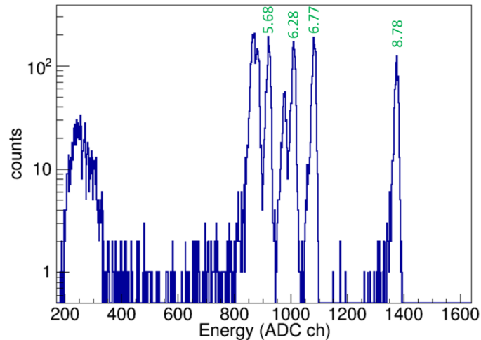
Figure 3: Alpha spectrum of a uranium-232 radioactive source detected with one strip of HiRA. Alpha-particles in this energy range are completely stopped in the first detection stage of HiRA. Data is reported in uncalibrated ADC channels. Peaks correspond to well-identified alpha-transitions. The peak at around 300 ch is caused by gamma-rays emitted by the source.
