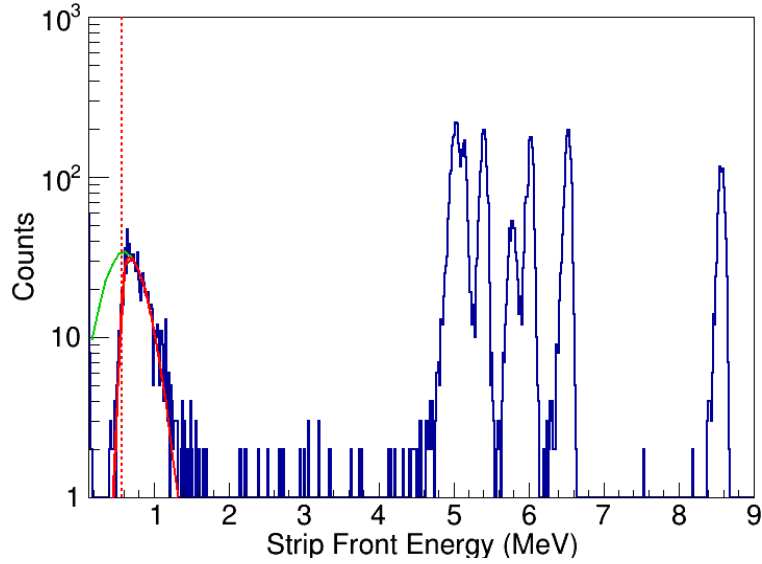
Figure 5: Fit of the gamma-peak observed with one front strip of HiRA. The fit is obtained with the combination of a Gaussian and a Fermi function (to simulate the effect of the detection threshold). The green curve shows the Gaussian function only as resulted from the fit. The red line is the global fit function. A red dashed line indicates the position of the deduced threshold.
